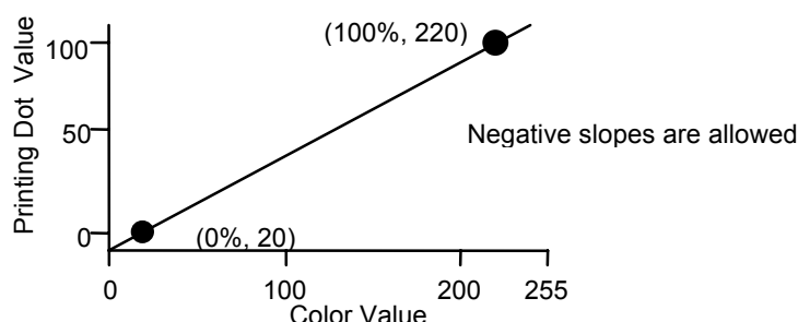
Figure 3 — Colour value versus print dot value
