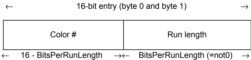
Figure 4 — Short form encoding structure in TIFF/IT-LW
